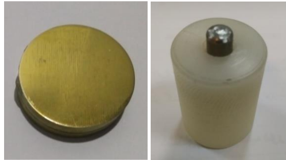
Fig. 7. Type I projectile with pin-shaped steel bullet (right) and TiN coated steel specimen (left)
