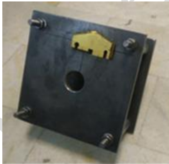
Fig. 6. View of the holding fixture of the sample in the impact test facility and how to fix the sample piece on the fixture
